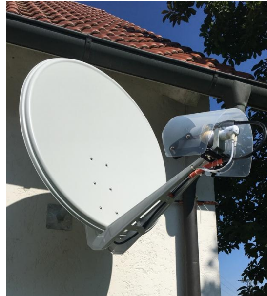
Dish d= 1m, Duo-Feed (Helix ANT + LNB )
